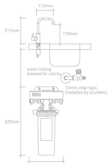
Tap hole size 22mm B-1000 Preferred installation layout
