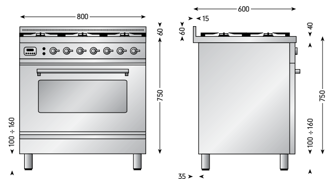
Model P 80 WMP Gas consumption: 61MJ/h Total electrical load: 3.7kW
