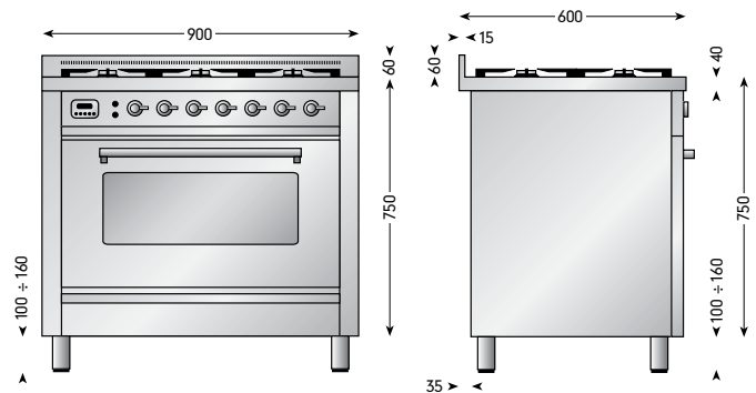
Electric oven Model P 90 WMP Gas consumption: 55MJ/h Total electrical load: 3.7kW
