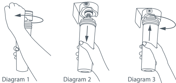
Fig.25 Changing the water filter cartridge
